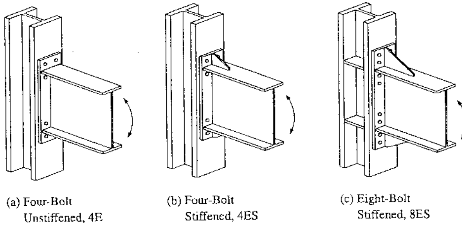
Extended end-plate configurations.
